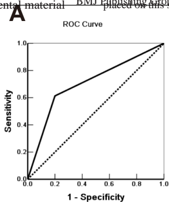
Figure S3 ROC curves of EphA10 (A) and Gli3 (B) in invasive breast cancer
